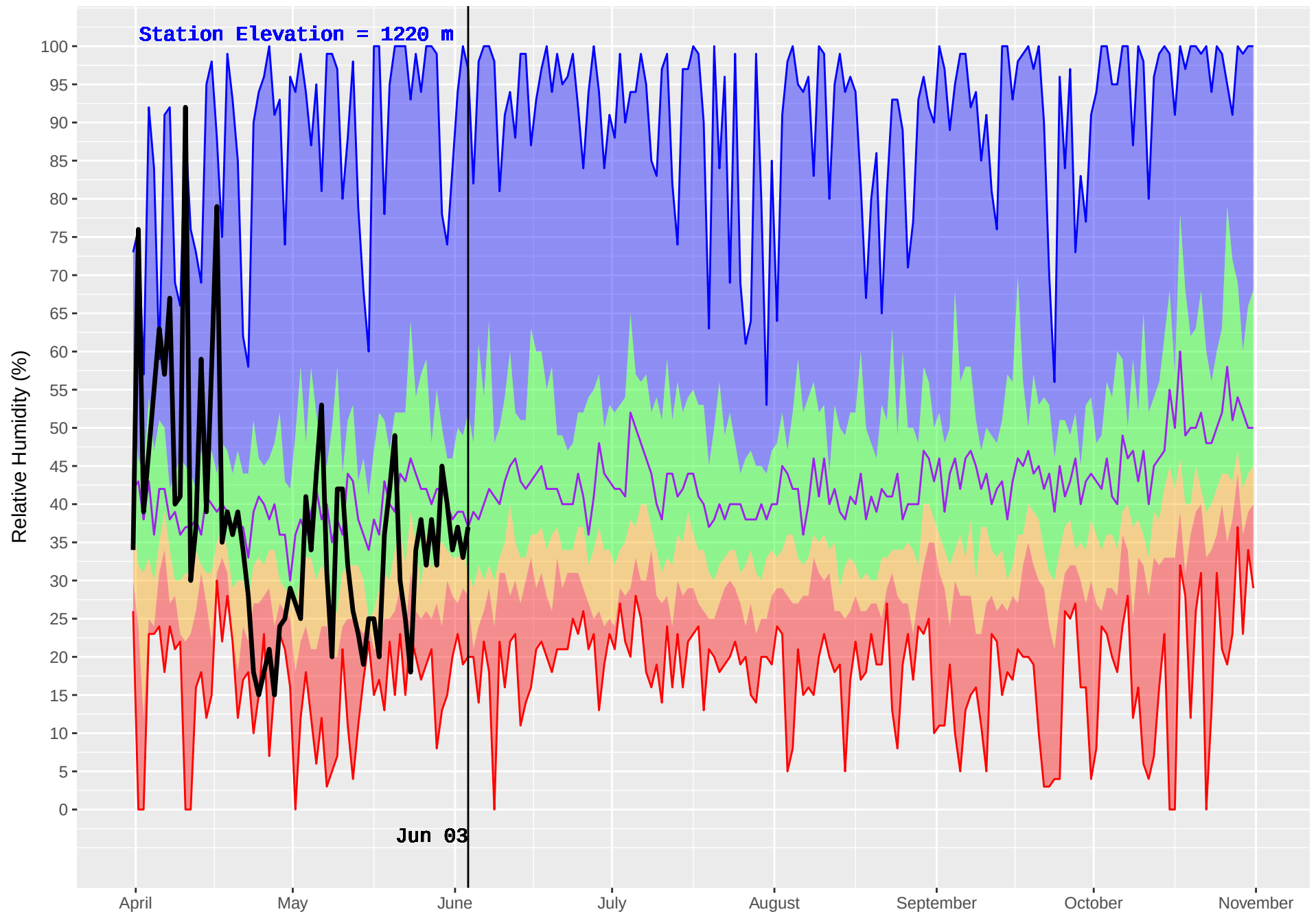
NEMIAH (216) : Historical (1982–2016) and Current (2018) Noon Relative Humidity
