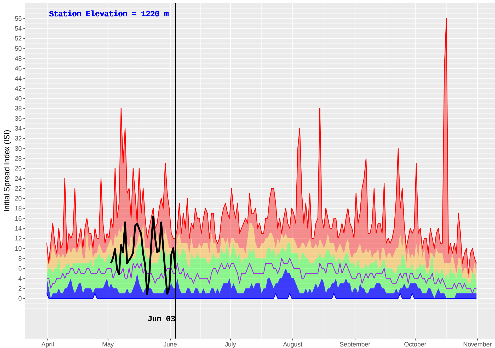
NEMIAH (216) : Historical (1982–2016) and Current (2018) Noon Initial Spread Index (ISI)
